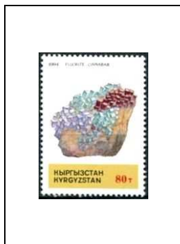
Fluorite - Cinabre
