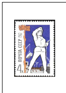
Docker
